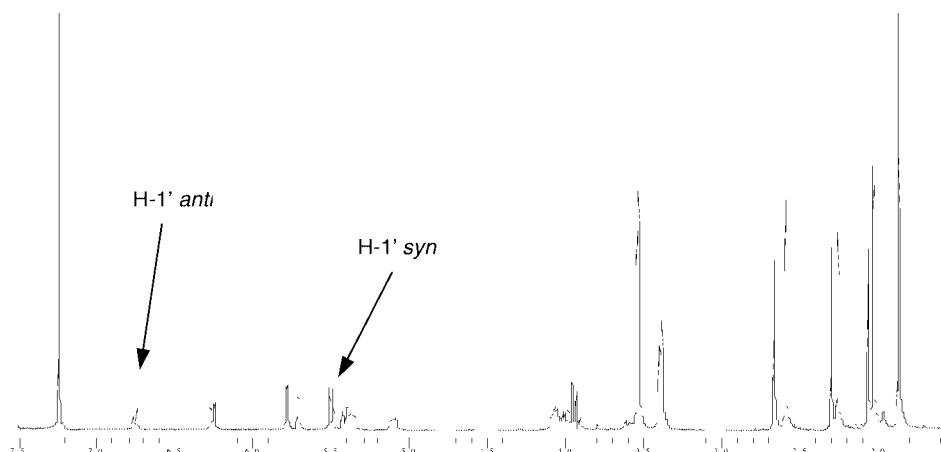
Figure 2. ^1\text{H} NMR ( \text{CDCl}_3 ) for compound 2 (263 K)
